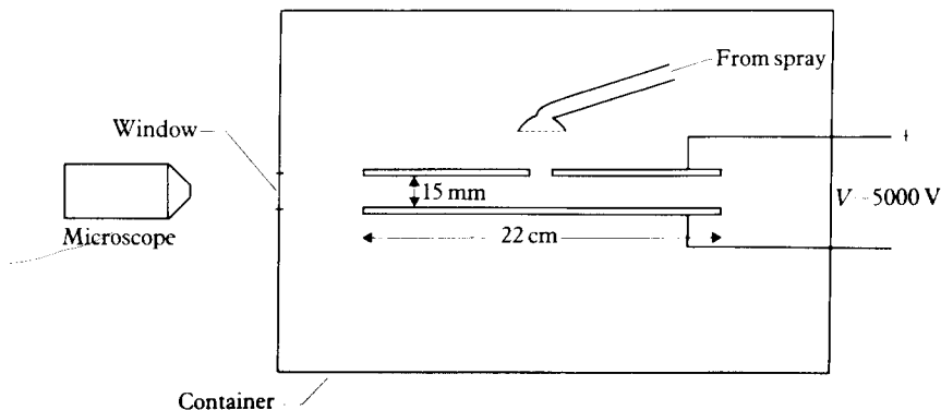
1.3 Millikan's experiment for the determination of the charge of the electron.
